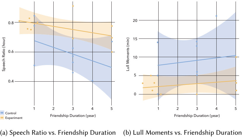
Fig. 7. The interaction between Speech Ratio/Lull Moments and Friendship Duration
