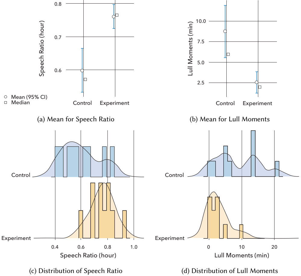
Fig. 6. The mean and the population distribution for Speech Ratio and Lull Moments.
