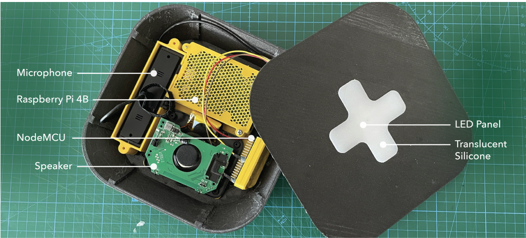
Fig. 3. Internal components and layout of the Boost prototype. Key parts are labeled, including the Raspberry Pi 4B, NodeMCU, microphone, speaker, LED panel, and translucent silicone cover.
